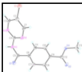
Fig. 1. Crystal structure of the title compound with atom labeling and displacement ellipsoids drawn at the 30% probability level.
