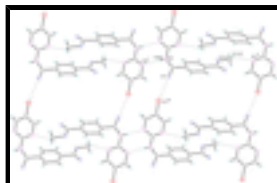
Fig. 2. Partial packing diagram showing C—H···N and N—H···N hydrogen bonds and C—Cl···O interactions among the molecules, with atom labeling and displacement ellipsoids drawn at the 30% probability level. Symmetric code: (i) 1 - x, 2 - y, -z; (ii) 1 - x, 1 - y, 1 - z; (iii) 1 + x, 1 + y, z.
